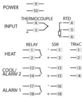
Wiring Connections*
